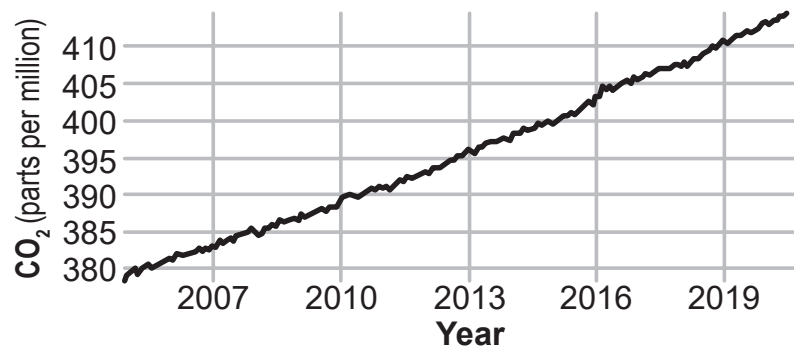
Graph 2: Atmospheric Carbon Dioxide
