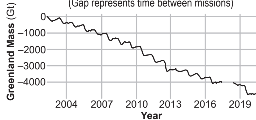
Graph 3: Greenland Mass Variation 2002 to 2020
